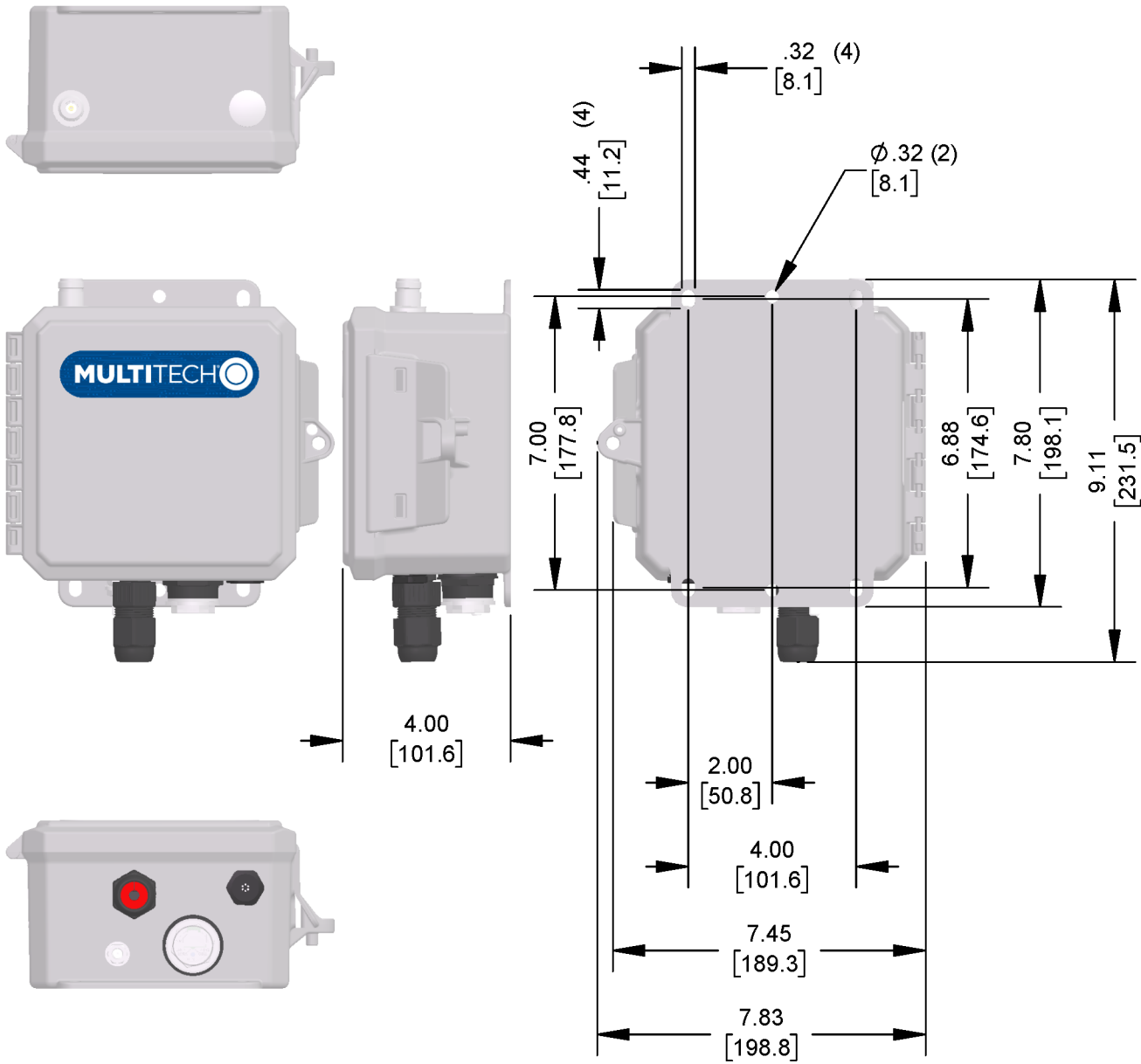
DIMENSIONS IN In [mm]
